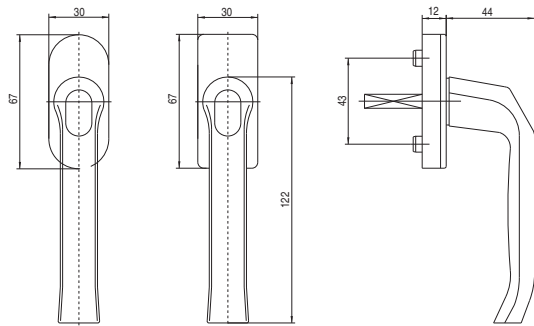
Klamka okienna
