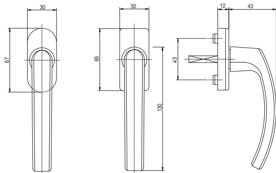
Klamka okienna
